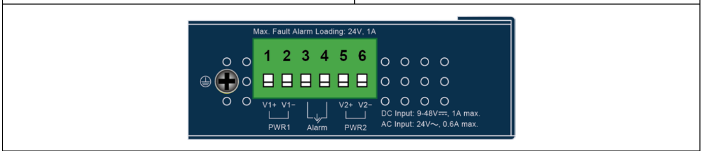
Figure 2-1-6: IGS-4215-4T2S Top View
