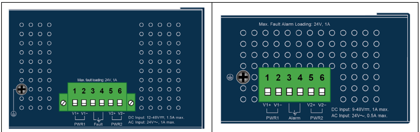
Figure 2-1-4: IGS-4215-16T2S Top View
