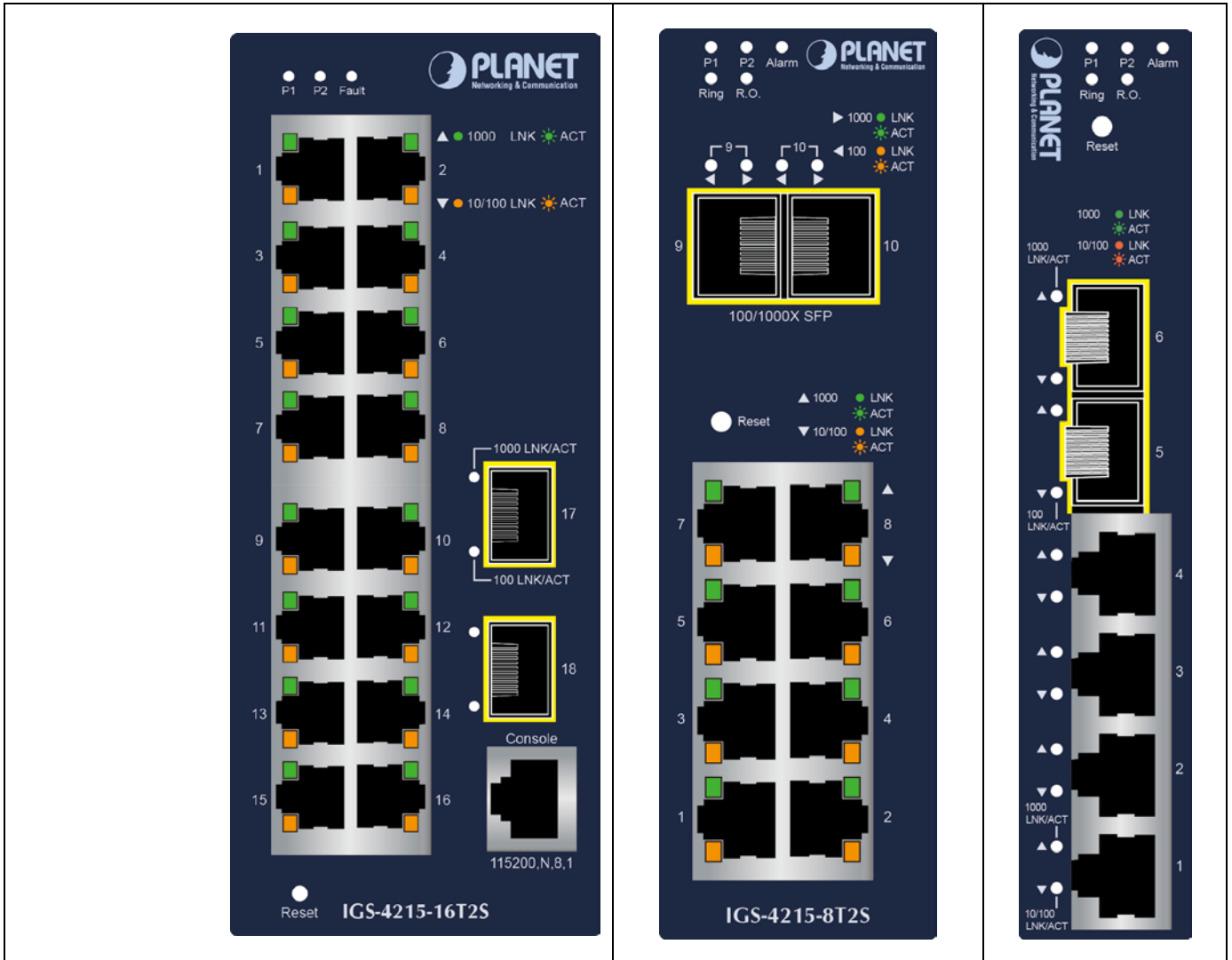
Figure 2-1-3: IGS-4215-16T2S / 8T2S / 4T2S LED Panel
